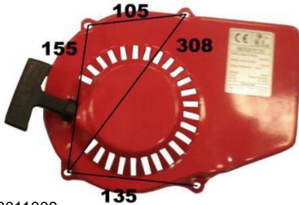
ARRANQUE COMPLETO GXH50, GXU50 .
