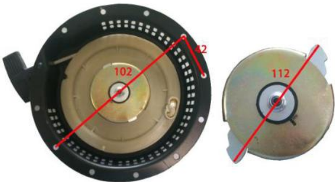
ARRANQUE COMPLETO 186F/LA100/LA-90
