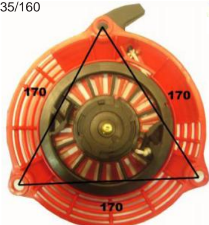
TAPA ARRANQUE COMPLETA OHV GC/GCV135/160
