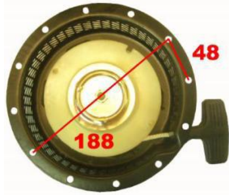
ARRANQUE YANMAR L60
