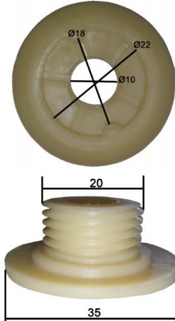
PIÑON BOMBA ENGRASE MOTOSIERRA 18", 45", 46", 52"
